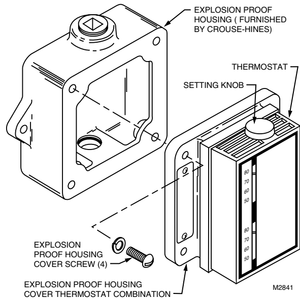
Fig. 2—Mounting T6051B Explosion Proof Heavy Duty Thermostat.
