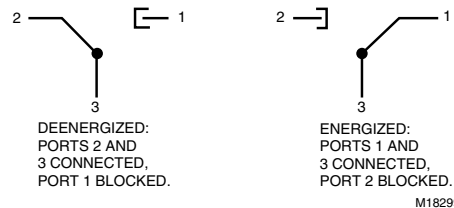
Fig. 7. Pneumatic schematic.
