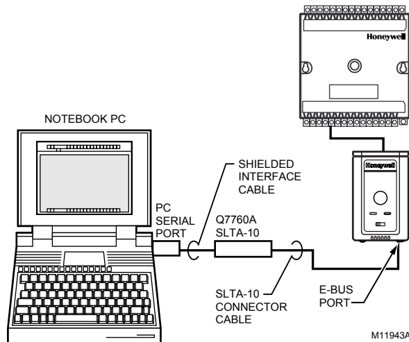
Fig. 14. Connecting the portable operator terminal to the LONWORKS® Bus.
