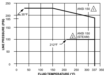
Fig. 1. Temperature-Pressure curves for V5011N and V5013N Valves.
