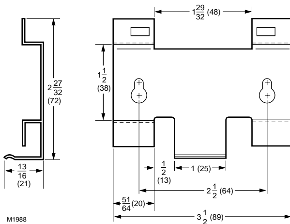
Fig. 1. 203765 Remote Mounting Bracket dimensions in in. (mm).
